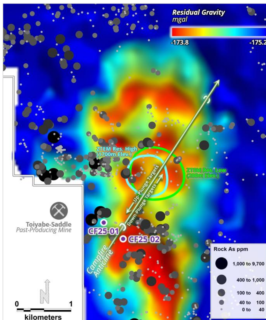
Figure 13: Holes CF25-01 & CF25-02 (Campfire Target, Toiyabe Hills Property)
